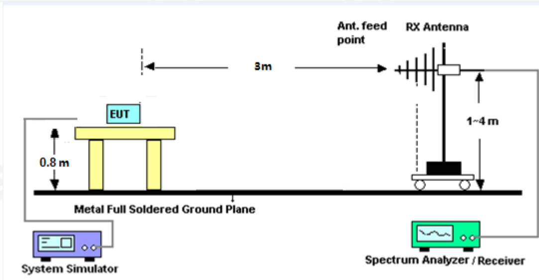
(A) Radiated Emission Test-Up Frequency Below 1 GHz
