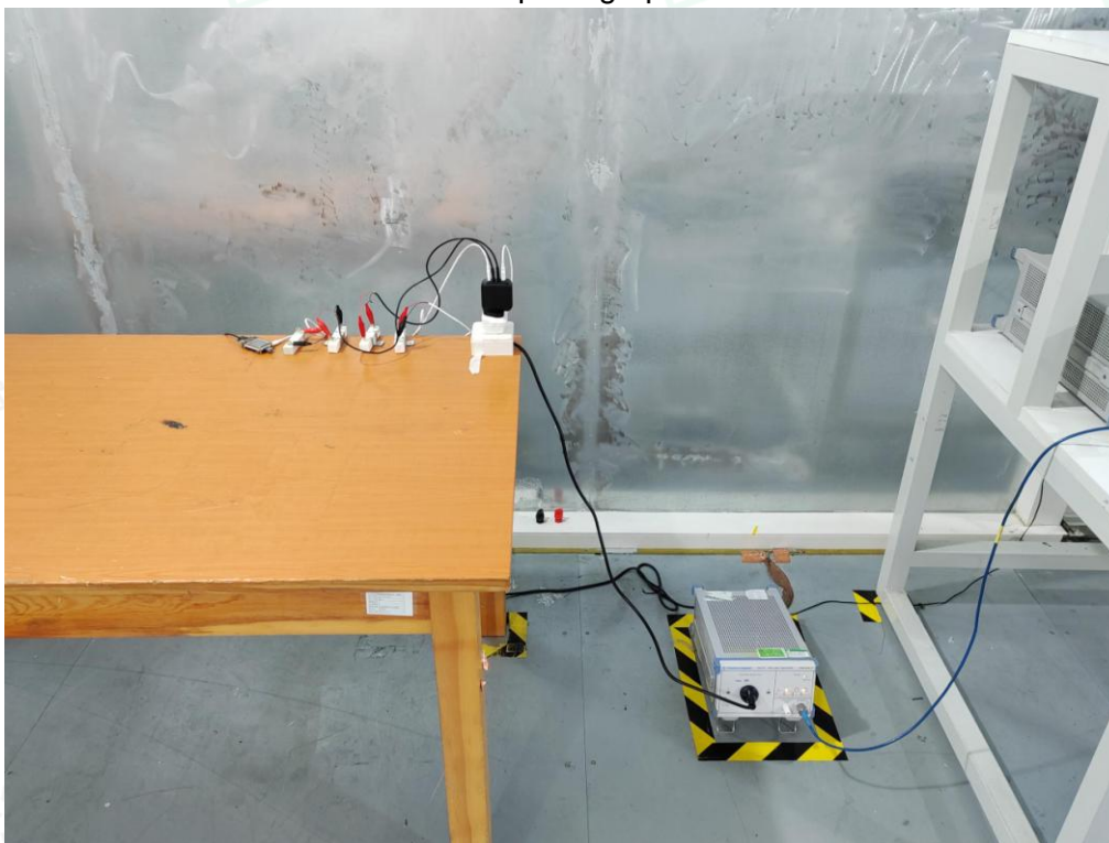
Test Setup Photo of Power Line Conducted Measurement
